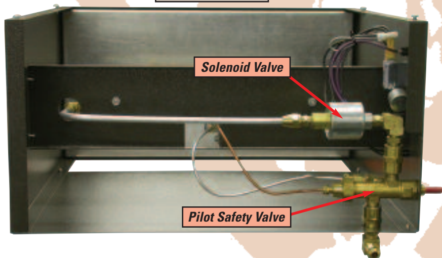
Bottom View
